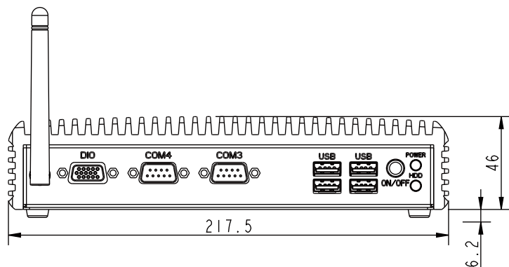
Rear View
