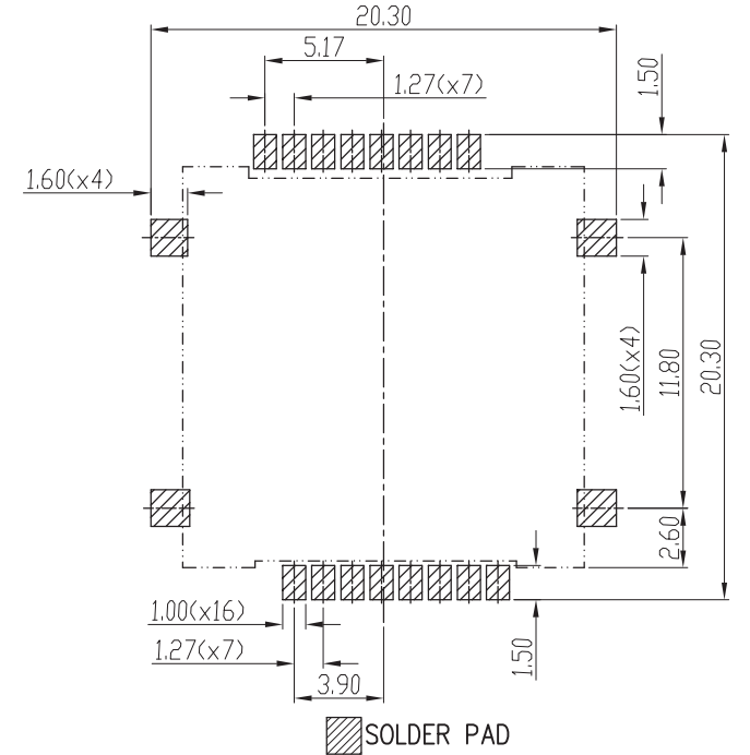
RECOMMENDED PCB LAYOUT TOLERANCE: ±0.05
