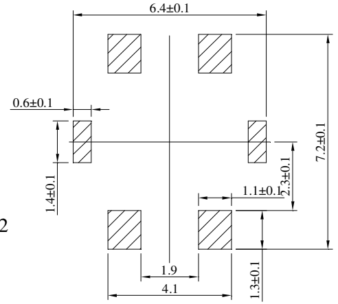
P.C.B mounting hole dimensions
